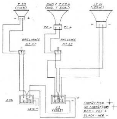
Fig. 3 — Schematic Wiring Diagram Separate 3-way System
